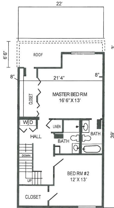
SECOND FLOOR LAYOUT
