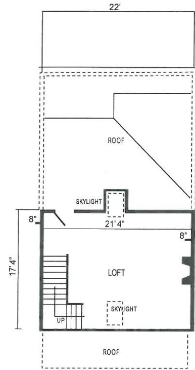
THIRD FLOOR LAYOUT "LOFT"
